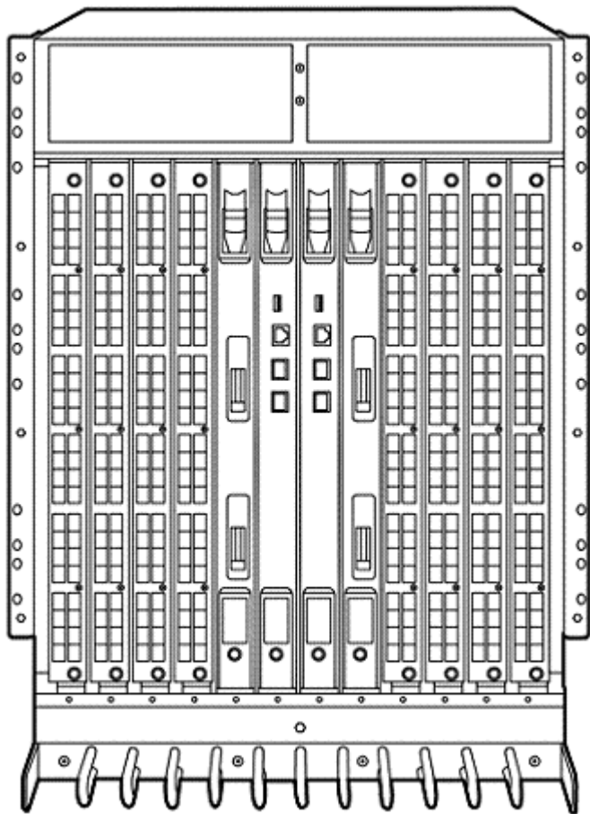
HP SN8000B 8-Slot SAN Director and DC SAN Backbone Director (shown) (identical chassis with different core blades and Fibre Channel blades)
